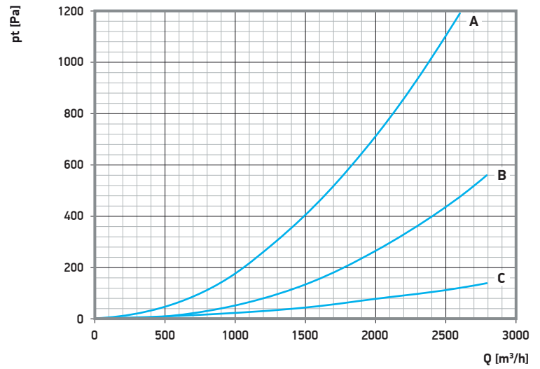
A - duct connector top DN 200 mm B - duct connector end DN 160 mm C - extraction rail type TECHNORAIL / m
